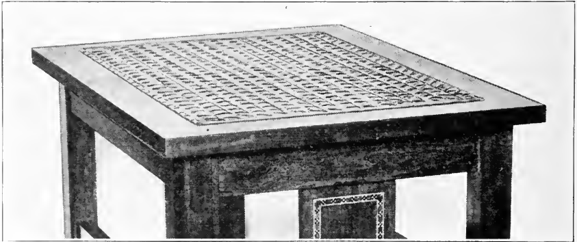
FIG. 495. COMPLETED SEAT.
